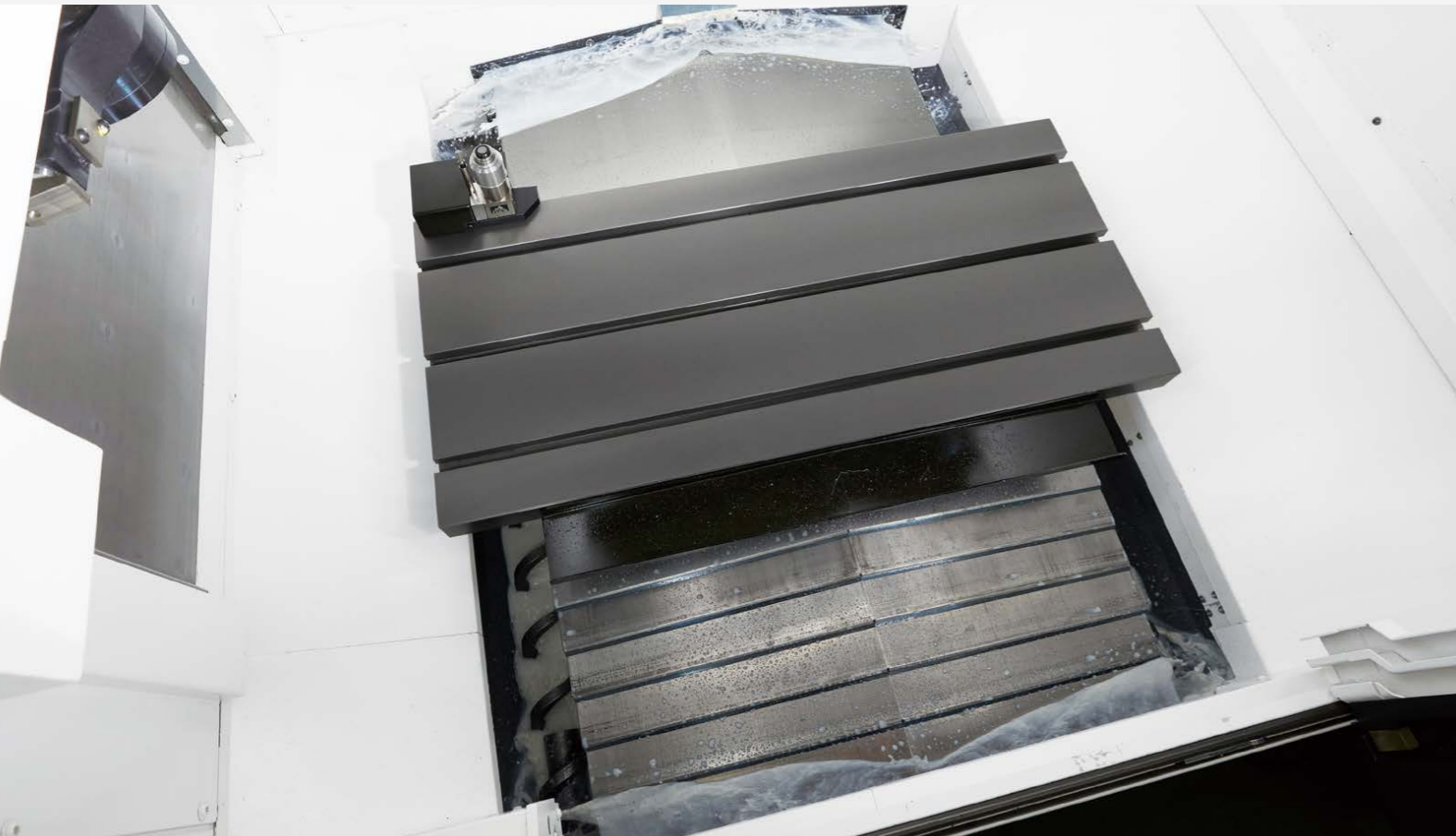
Photo shows the machining chamber of the MB-46VEII
